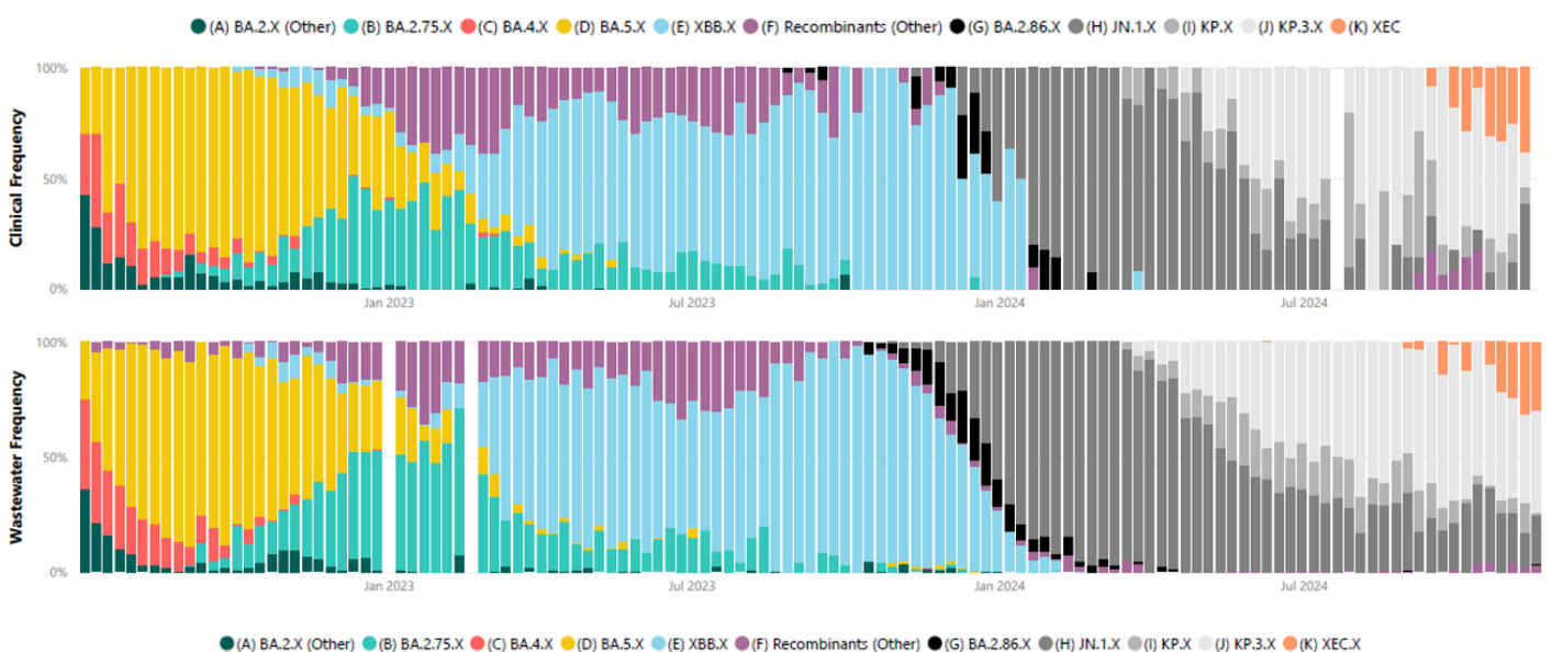
Figure 12. Distribution of SARS-CoV-2 variants in clinical samples (top) and metropolitan wastewater catchments (bottom), 03 July 2022 to 17 November 2024.
